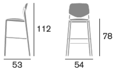
Dimensioni / Sizes (cm) A
