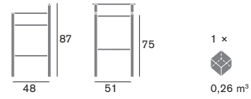
Penelope 2731 SG Dimensioni / Sizes
